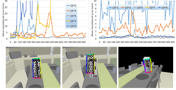
Figure 6. Top: Mean translational error for a changing \lambda on every 20th frame for 'kinect_box' (left) and 'tide' (right). Bottom: Tracking performance on 'kinect_box'. With \lambda = 10^5 , the balance between contour and interior points drives the pose correctly. With \lambda = 10^9 , the energy is dominated by the plane-to-point ICP term, which leads to drifting for planar objects. With an emphasis on contour alone ( \lambda = 10 ), we deviate later due to an occluding cup.
