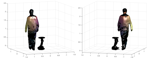
Fig. 11. Predicted data-model associations on noisy visual hulls with Hough forests. Black color means that the points are either outliers, or the inferred correspondences are rejected due to incompatible normals.
